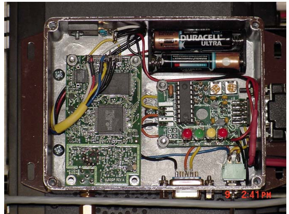
Internal layouts and wiring
